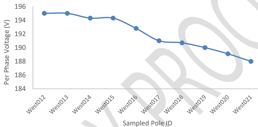
Figure 4: Measured Voltage Profile of West-End Network Leg 1
