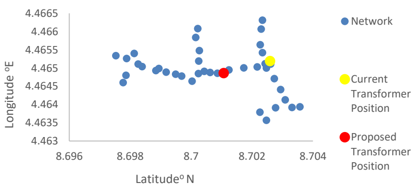
Figure 11: Safari2 Network Showing the Proposed Location of Transformer
