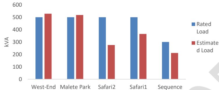
Figure 8: Comparison of Estimated Loading and Nominal Power of Transformers
